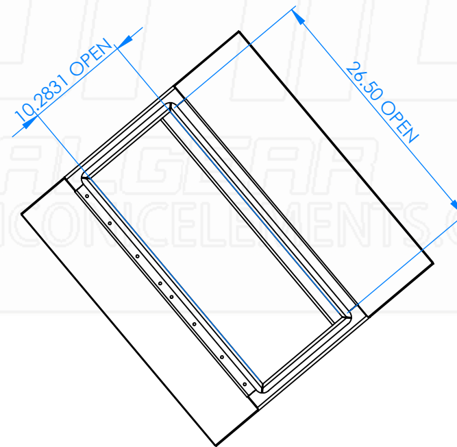
VIEW C SCALE 1 : 13
